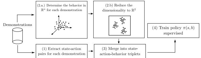
Fig. 1. Behavioral Repertoire Imitation Learning (BRIL) trains a policy \pi(s, b) supervised on a data set of state-action pairs augmented with behavioral descriptors in \mathbb{R}^2 for each demonstration. When deployed, a system can adapt its behavior by modulating b . High-dimensional behavioral spaces can be reduced using dimensionality reduction, as low-dimensional behavioral descriptions allow for faster adaption.
